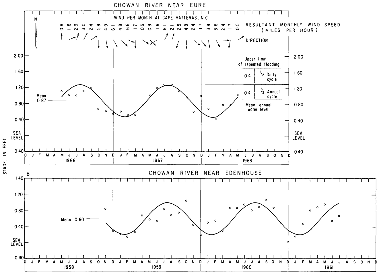
Figure 4.19. Monthly average stages for Chowan River near Eure and Chowan River near Edenhouse. The solid lines are sine curve approximations of the annual cycle of water levels (From Daniel, 1977)
