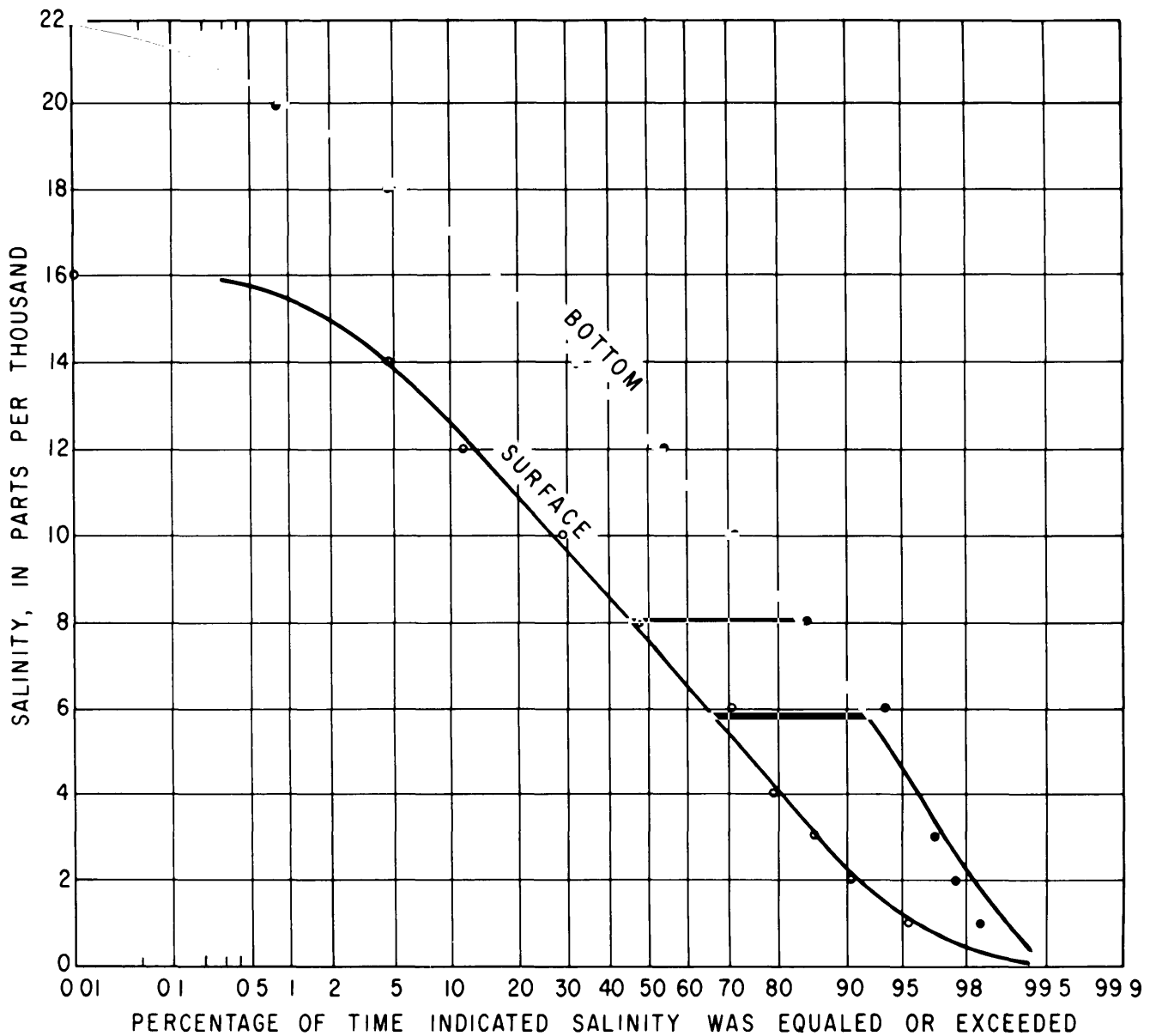
Figure 3.23. Percentage of time surface and bottom salinities were equaled or exceeded in the Neuse River estuary at Wilkinson Point Light, 1958-67. Data are from the University of North Carolina Institute of Marine Sciences, Morehead City, N.C., and the Carolina Power and Light Company.
