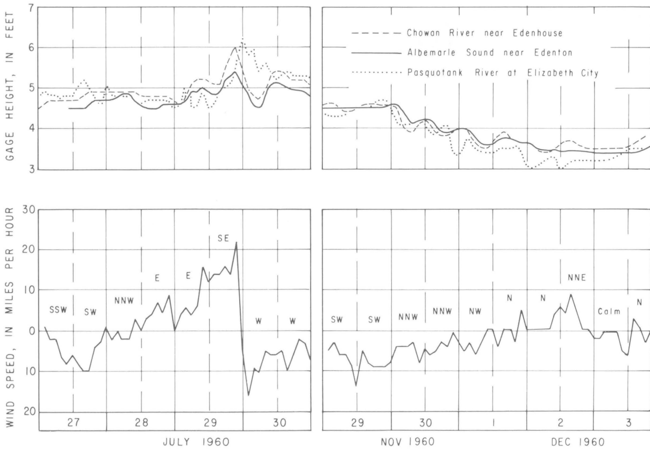
Figure 4.3. Wind speed at Elizabeth City and water levels at Chowan River near Edenhouse, Albemarle Sound near Edenton, and Pasquotank River at Elizabeth City, July 27–30 and November 29–December 3, 1960. Water level records are from tide gages operated by U.S. Army Corps of Engineers.
