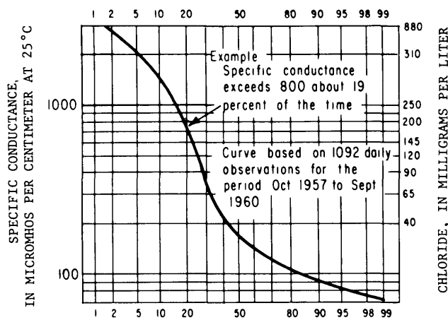
PERCENTAGE OF TIME SPECIFIC CONDUCTANCE OR CHLORIDE CONCENTRATION IS EQUAL TO OR GREATER THAN A GIVEN VALUE
