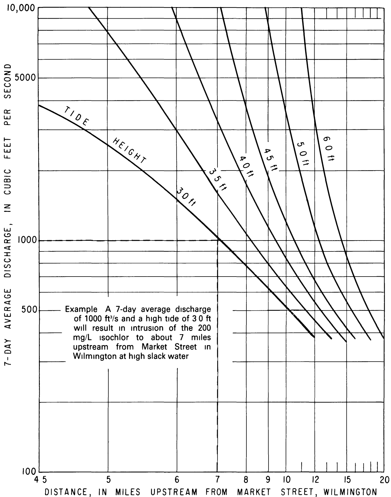
Figure 2.11. Interrelations of maximum encroachment of 200 mg/L chloride, outflow at the mouth, and tide heights in the Cape Fear River estuary (Revised version of relation developed by Wilder and Hubbard, 1968 )
