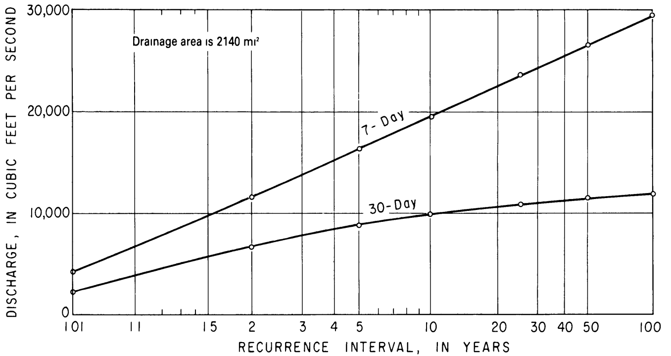
Figure 3.33. Maximum 7- and 30-consecutive-day average discharges of the Tar River at Tarboro
