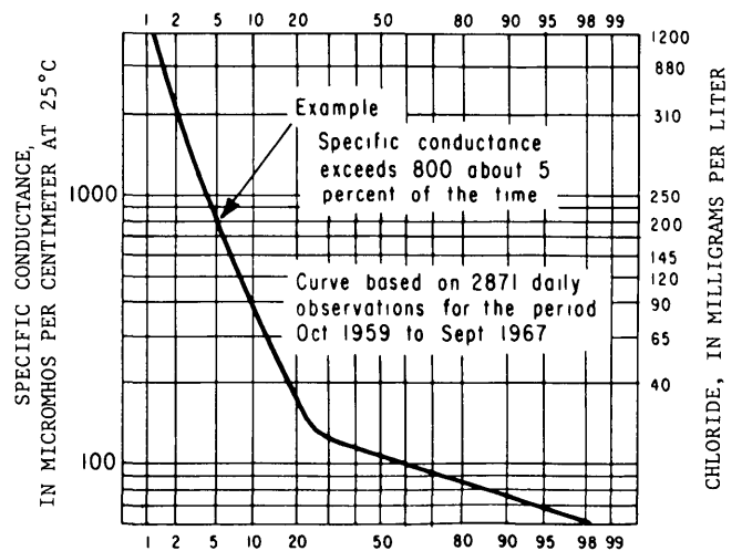
PERCENTAGE OF TIME SPECIFIC CONDUCTANCE OR CHLORIDE CONCENTRATION IS EQUAL TO OR GREATER THAN A GIVEN VALUE
