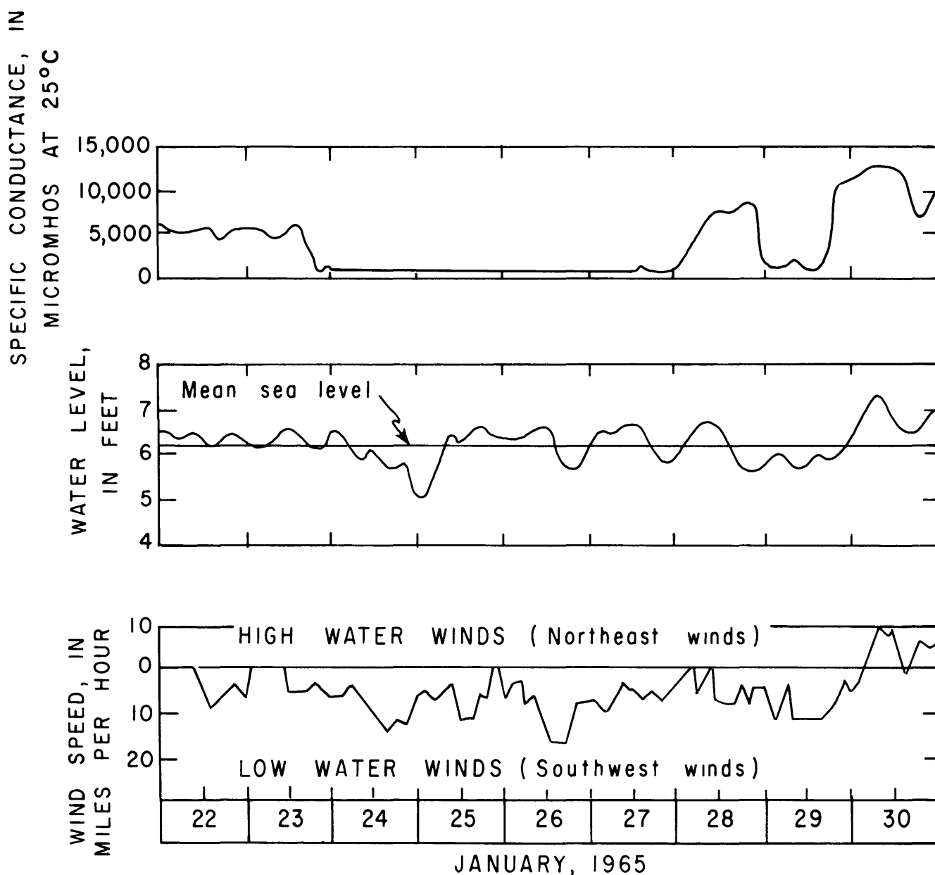
Figure 3.15. Effect of wind on water levels and bottom specific conductance in the Neuse River estuary at New Bern, January 22-30, 1965. Datum of water level gage is -6.15 ft MSL.
