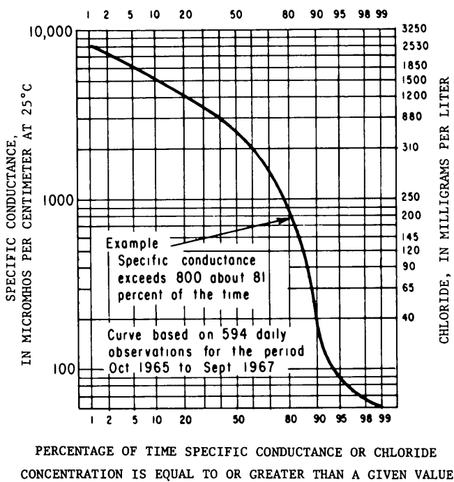
Figure 4.15 Cumulative frequency curve of specific conductance and chloride, Scuppernon River at Columbia (sta 02081172 on pl 1) (From Wilder and others, 1978 )
