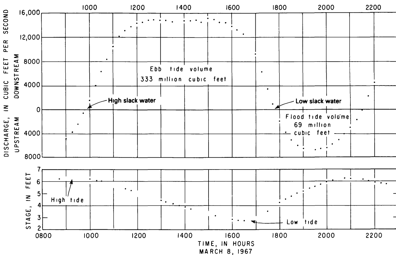
Figure 2.4. Stage and discharge of the Cape Fear River estuary near Phoenix on March 8, 1967
