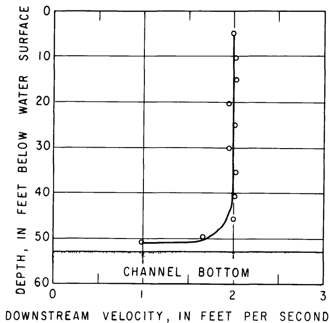
Figure 2.5. Variation of velocity with depth of the Cape Fear River estuary at Navassa on May 13, 1966 (at meter station 20, 0759-0803 hours)
