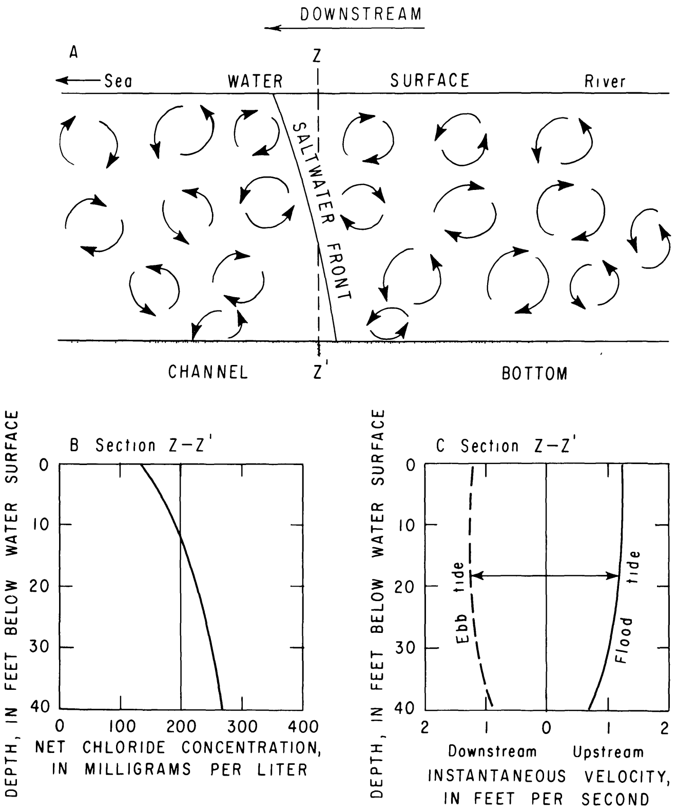
Figure 1.8 A Net circulation patterns in a well mixed estuary B Chloride concentration profile through section Z-Z' C Velocity profiles through section Z-Z'
