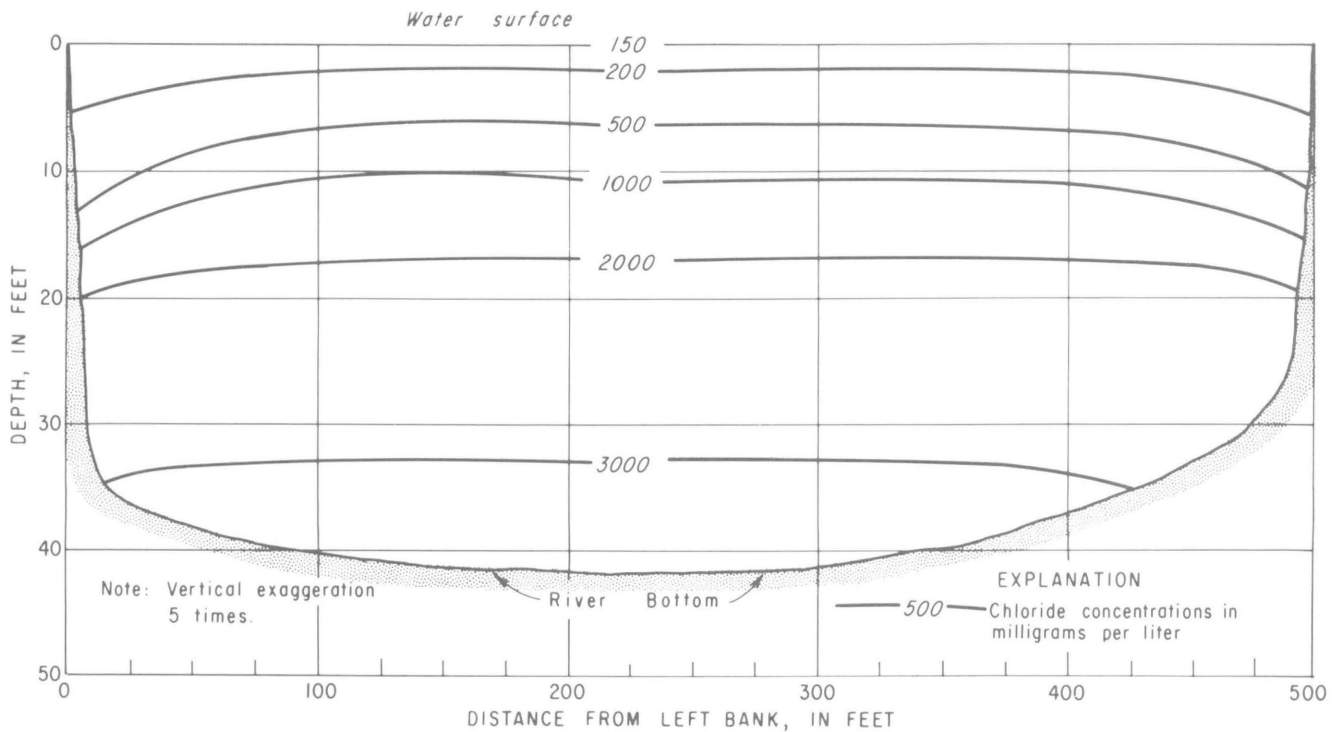
Figure 2.7. Variations in chloride concentrations in a cross section of the Cape Fear River estuary 1.5 miles upstream from Market Street, Wilmington, on June 5, 1962. (From Wilder and Hubbard, 1968.)
