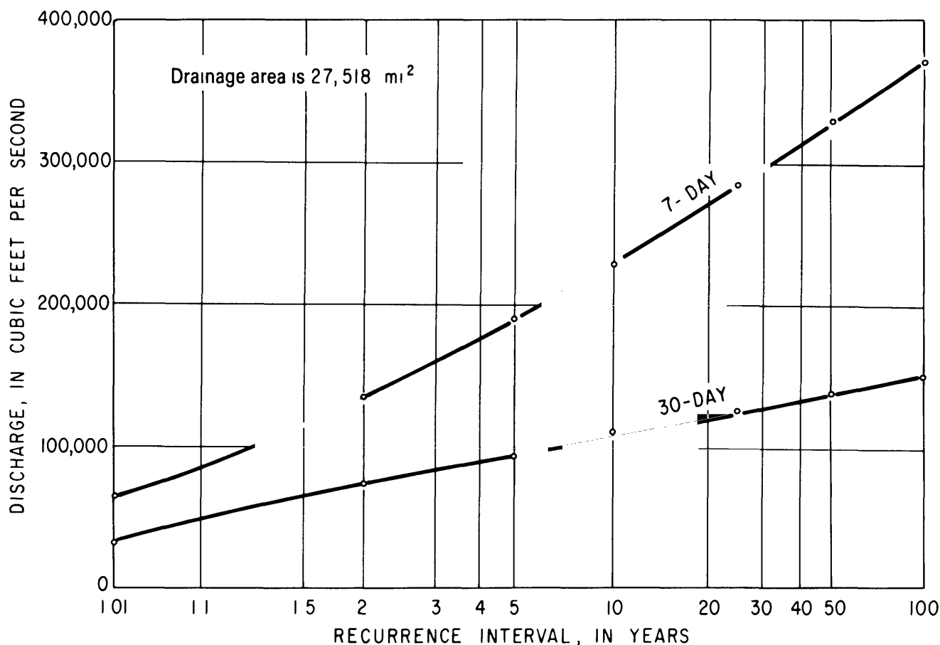
Figure 3.6. Magnitude and frequency of annual maximum 7- and 30-consecutive-day average inflow to Pamlico Sound from direct and indirect land drainage, not adjusted for precipitation on and evaporation from Pamlico and Albemarle Sounds and associated open-water areas. The total area not adjusted for is 3,362 square miles of the total drainage area of Pamlico Sound of 30,880 square miles.
