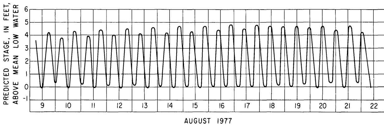
Figure 1.1. Tide curve for Cape Fear River estuary at Wilmington for August 9-22, 1977, based on predicted times and heights of high and low water from National Ocean Survey Tide Tables
