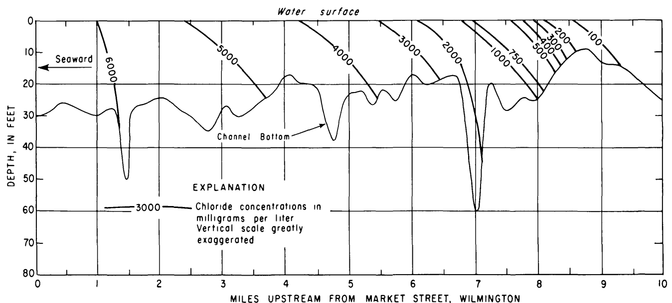
Figure 2.6. Longitudinal variations in chloride concentrations of the Cape Fear River estuary at high-slack water, November 1, 1967 (From Wilder and Hubbard, 1968) (Refer to fig. 2.3 for locations.)
