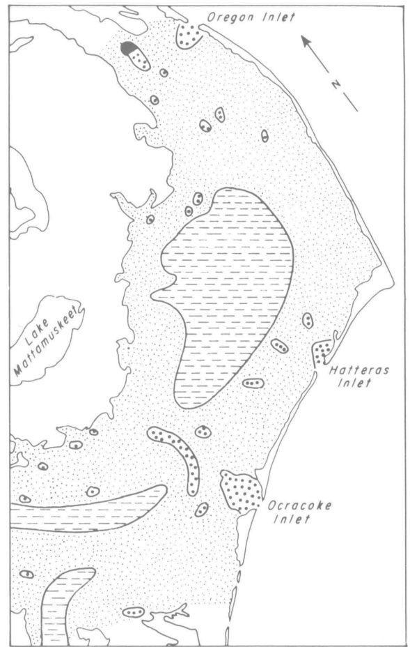
EXPLANATION ■ Coarse sand ● Medium sand ○ Fine-very fine sand ▨ Silt
