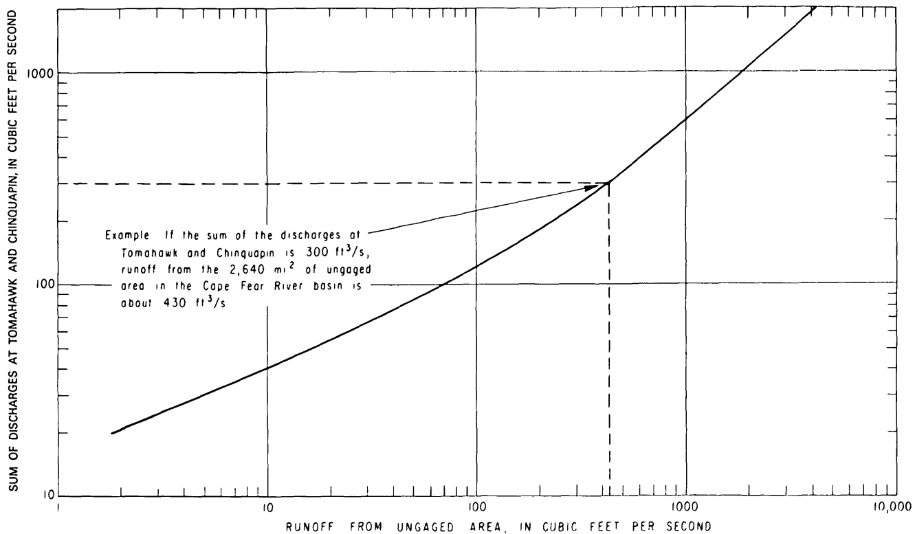
Figure 2.1. Concurrent discharge relation for estimating runoff from the ungauged drainage area between the index stations and the mouth of the Cape Fear River estuary (Modified from Wilder and Hubbard, 1968)
