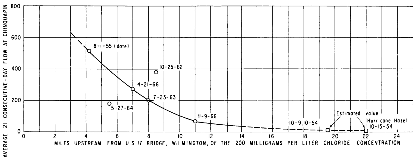
Figure 2.19 Relation of the location of the saltwater front in the Northeast Cape Fear River estuary to the preceding 21-day average discharge at Chinquapin
