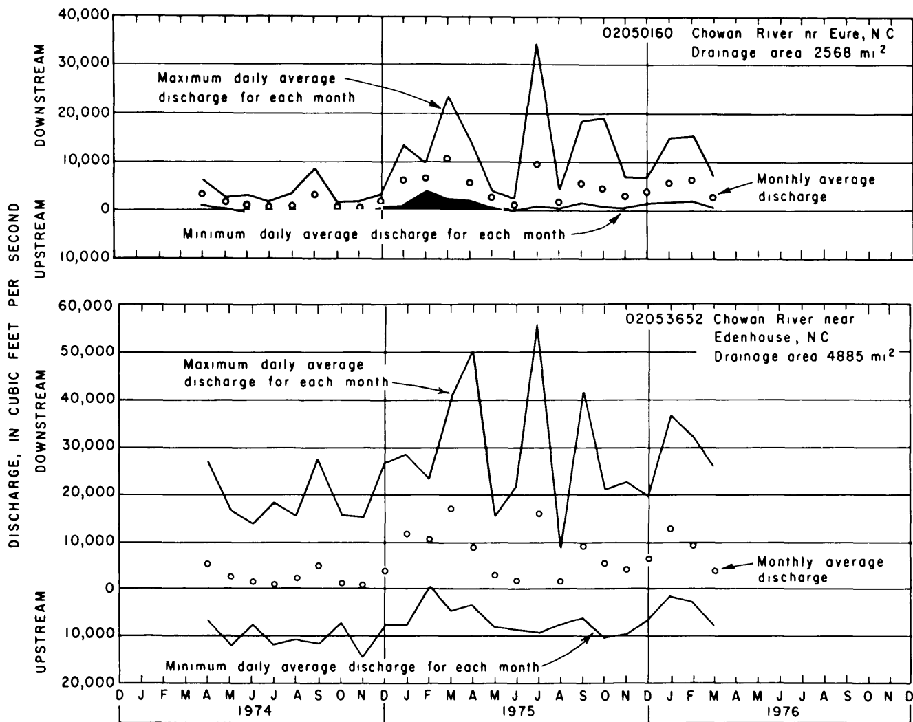
Figure 4.22 Monthly average discharge and maximum and minimum daily average discharge of Chowan River near Eure and Chowan River near Edenhouse (From Daniel, 1977 )
