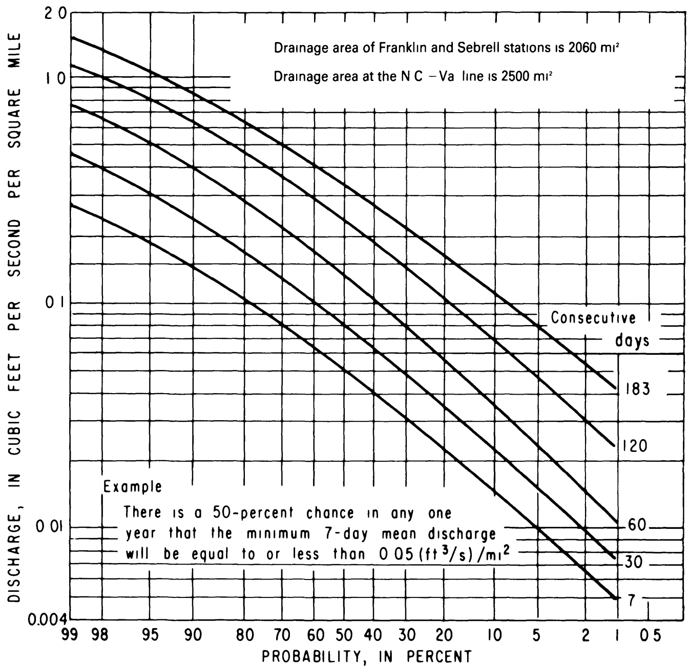
Figure 4.21. Low-flow frequency curves of annual lowest mean discharge for indicated number of consecutive days, combination of Blackwater River at Franklin, Va and Nottoway River at Sebrell, Va (From Wilder and others, 1978 )
