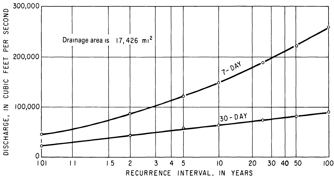
Figure 4.5. Maximum 7- and 30-consecutive-day average inflow to Albemarle Sound from land drainage (not adjusted for precipitation on and evaporation from open-water areas)
