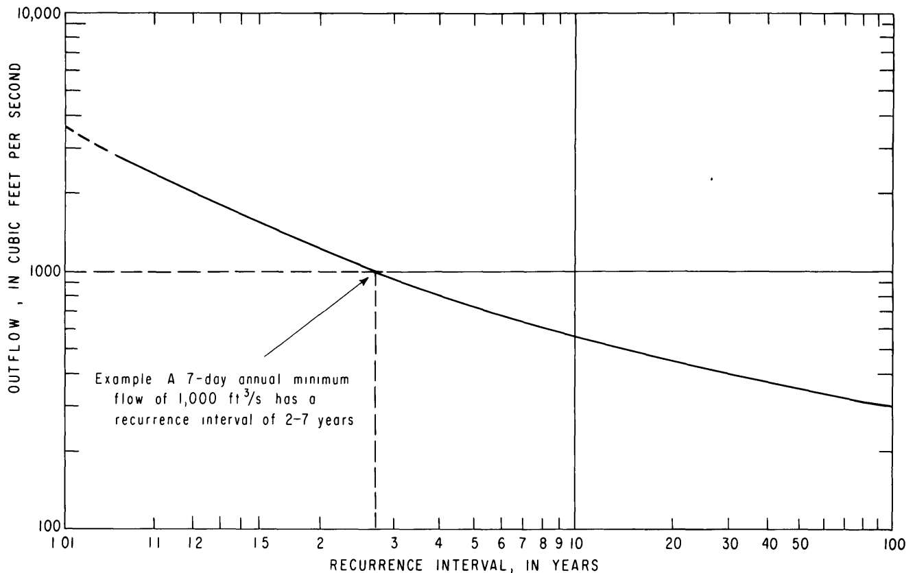
Figure 2.2. Magnitude and frequency of annual minimum 7-day average net flow of the Cape Fear River estuary at the mouth, near Southport
