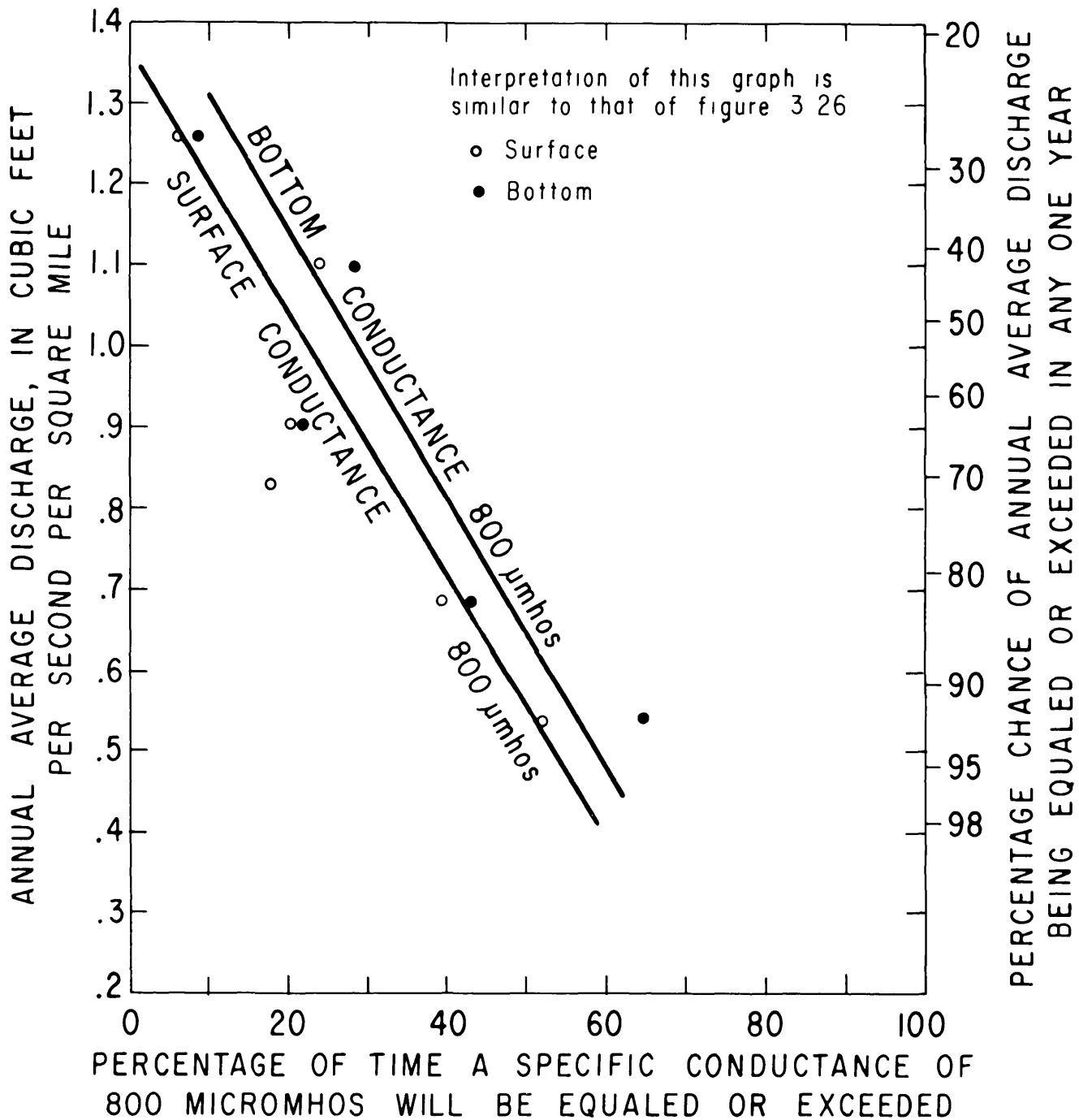
Figure 3.38 Percentage of time a specific conductance of 800 \mu mhos will be equaled or exceeded in the Pamlico River at Washington for various annual average discharges at Tarboro (drainage area—2,140 mi^2 )
