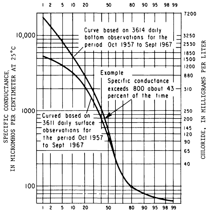
PERCENTAGE OF TIME SPECIFIC CONDUCTANCE OR CHLORIDE CONCENTRATION IS EQUAL TO OR GREATER THAN A GIVEN VALUE
