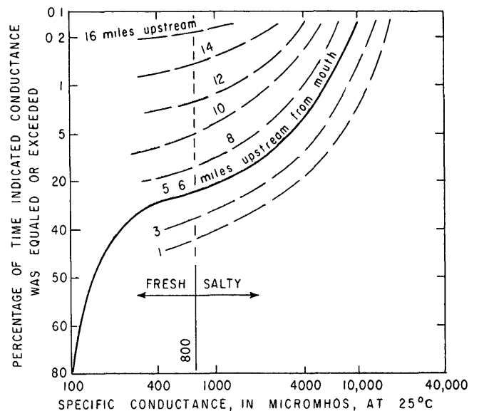
Figure 3.21. Percentage of time that integrated specific conductances were equaled or exceeded for several locations in the Trent River estuary, 1959-61.
