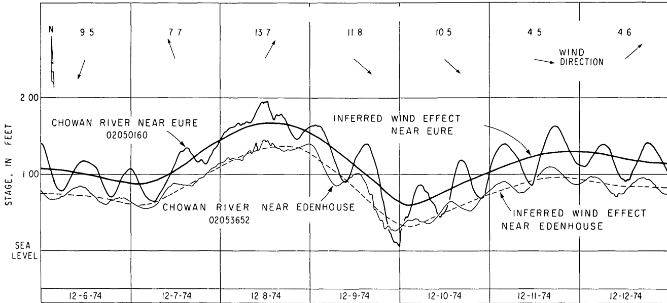
AVERAGE DAILY WIND SPEED AND DIRECTION, IN MILES PER HOUR AT CAPE HATTERAS, N C
