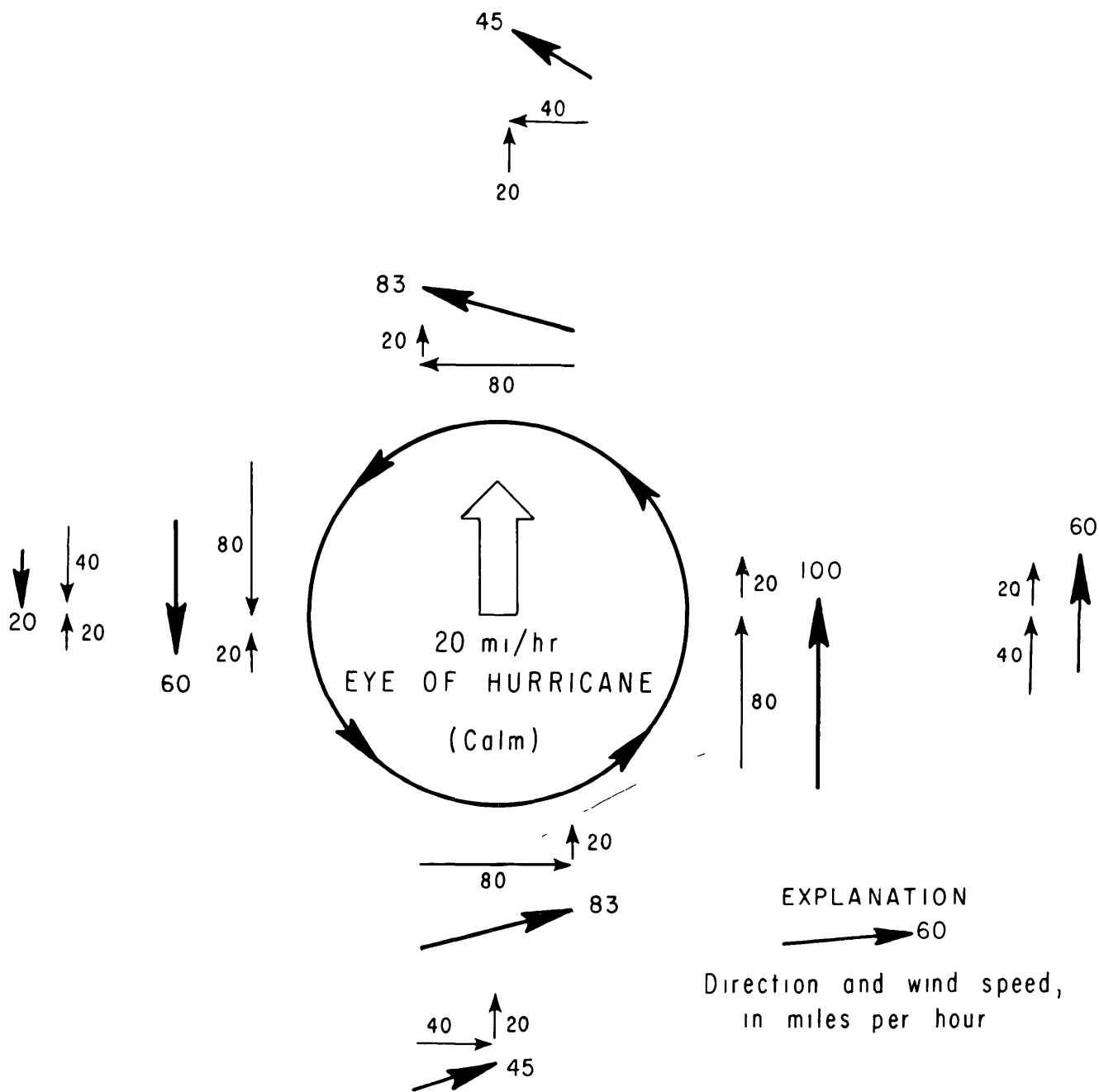
Figure 1.9 The effect of forward motion of a hurricane on wind velocities in each quadrant
