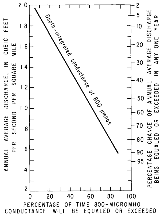
Figure 3.27. Percentage of time a specific conductance of 800 \mu\text{mhos} will be equaled or exceeded in the Trent River near New Bern for various annual average discharges at Trenton (drainage area—138 \text{mi}^2 )
