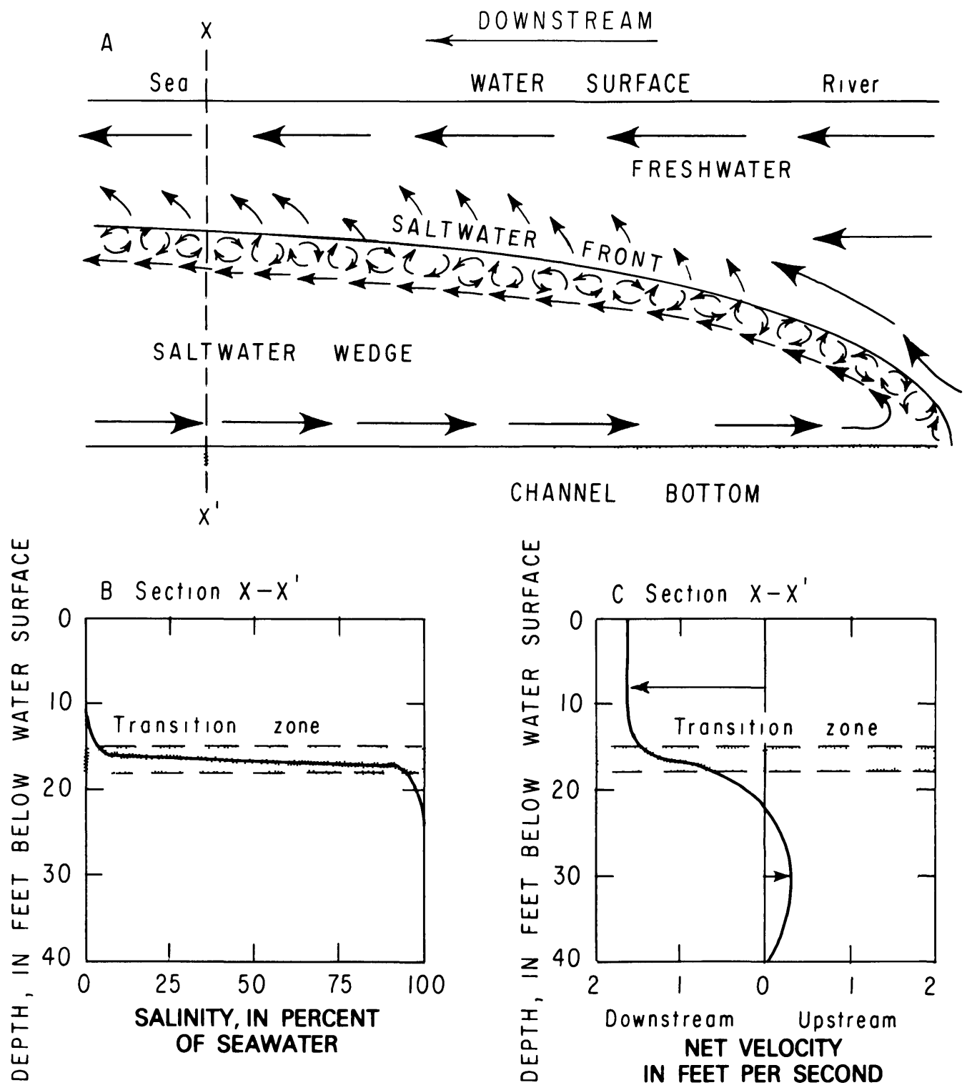
Figure 1.6. A Net circulation patterns in a highly stratified estuary B Salinity profile through section X-X' C Net velocity profile through section X-X'
