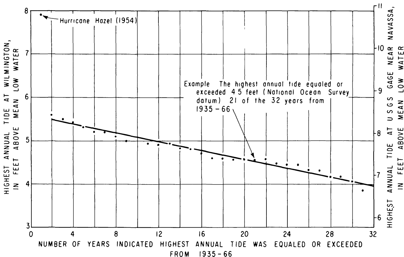
Figure 2.10. Magnitude and frequency of highest annual tide in the Cape Fear River estuary at Wilmington, corrected for component of river stage due to freshwater inflow (From Wilder and Hubbard, 1968)
