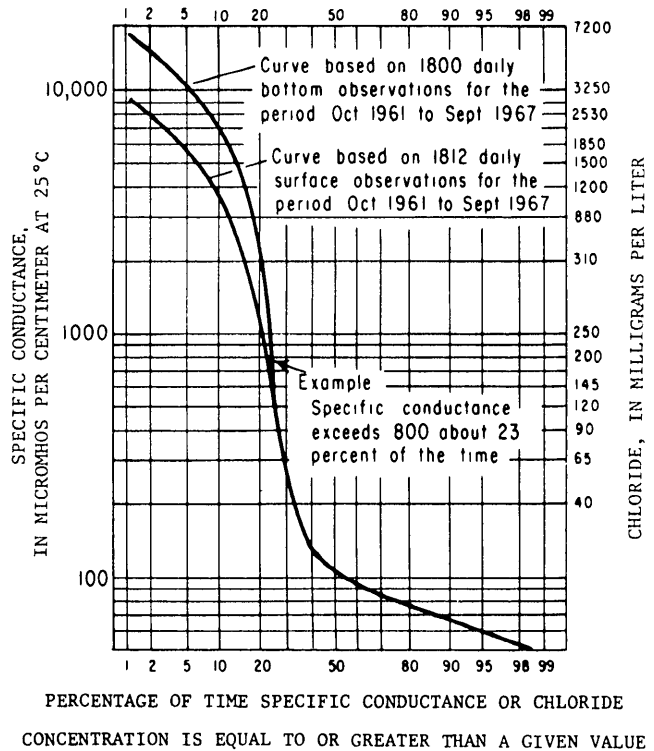
Figure 3.36. Cumulative frequency curves of specific conductance and chloride, Pamlico River at Washington (After Wilder and others, 1978 )
