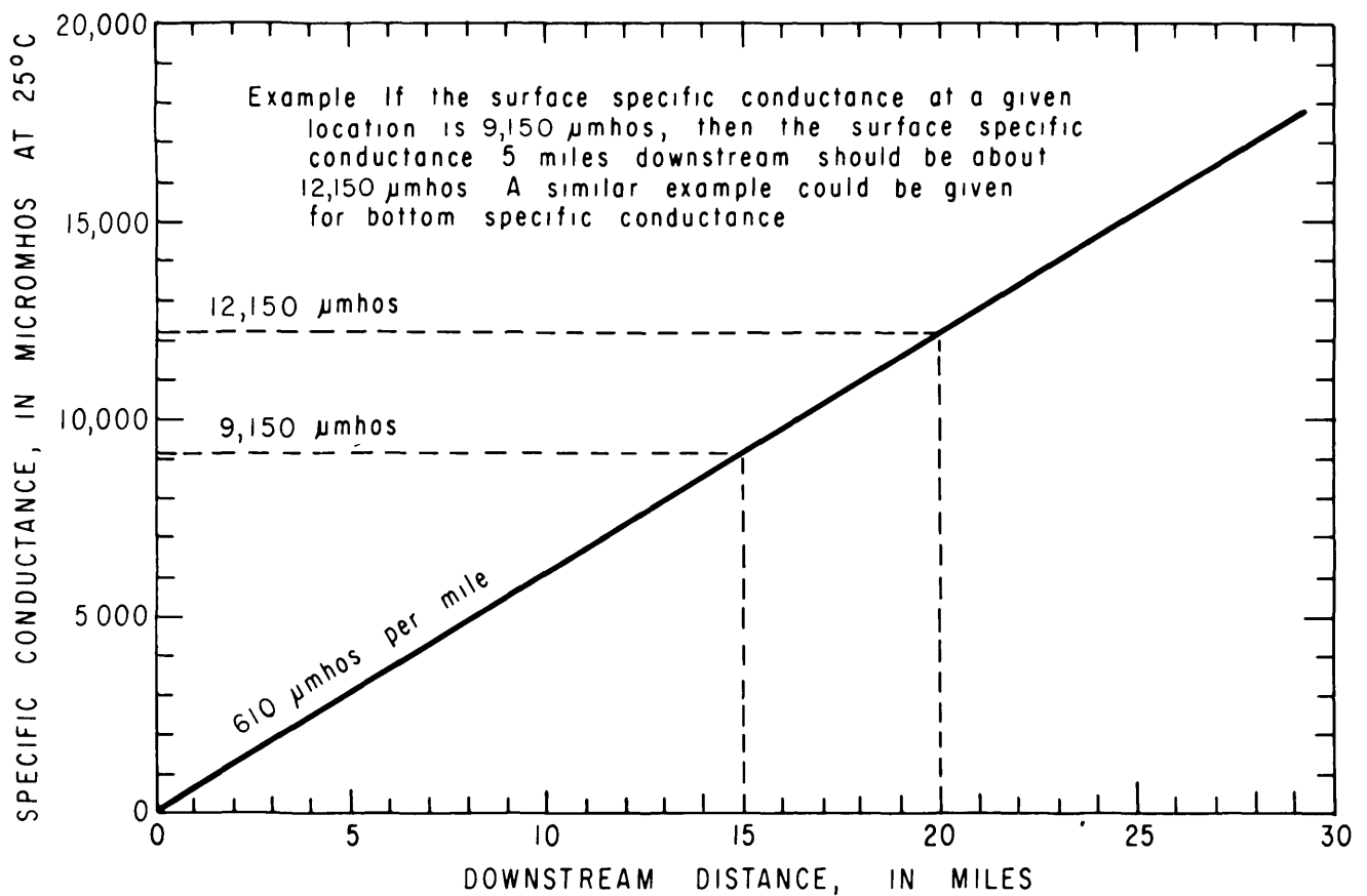
Figure 3.37. Relation between surface specific conductance at one point in the Pamlico River estuary and surface specific conductance at other points either upstream or downstream
