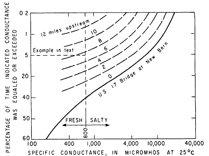
Figure 3.20. Percentage of time that surface specific conductances were equaled or exceeded for several locations in the Neuse River estuary, 1957-67.
