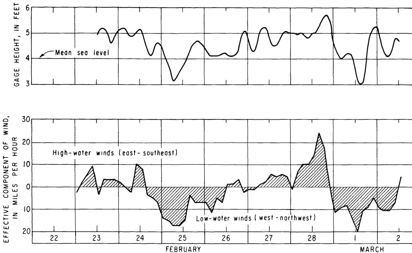
Figure 3.29. Water levels in the Pamlico River at Washington and effective component of wind speed at Cape Hatteras, February 22–March 2, 1966. Wind speeds are from National Weather Service records, water levels provided by the Corps of Engineers.
