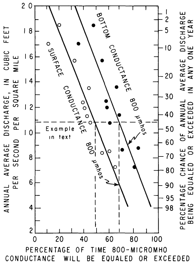
Figure 3.26. Percentage of time a conductance of 800 \mu\text{mhos} will be equaled or exceeded in the Neuse River at New Bern for various annual average discharges at Kinston (drainage area—2,690 \text{mi}^2 )
