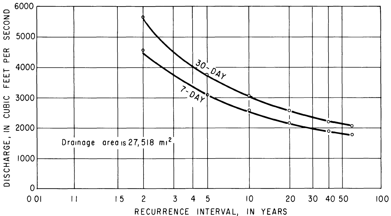
Figure 3.5 Magnitude and frequency of annual minimum 7- and 30-consecutive-day average inflow to Pamlico Sound from direct and indirect land drainage, not adjusted for precipitation on and evaporation from Pamlico and Albemarle Sounds and associated open-water areas
