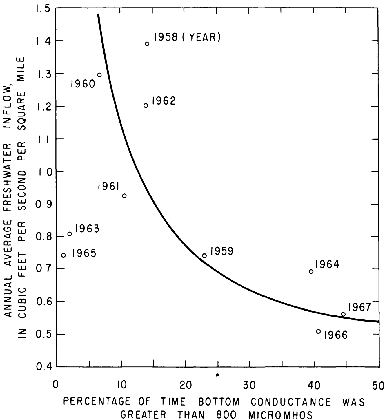
Figure 4.23. Percentage of time bottom specific conductances exceeded 800 micromhos for various annual average discharges for Chowan River near Edenhouse, 1958–67
