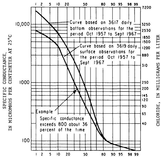
PERCENTAGE OF TIME SPECIFIC CONDUCTANCE OR CHLORIDE CONCENTRATION IS EQUAL TO OR GREATER THAN A GIVEN VALUE
