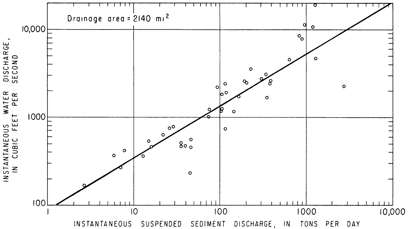
Figure 3.35. Sediment-transport curve for the Tar River at Tarboro, based on measurements made during 1974–76
