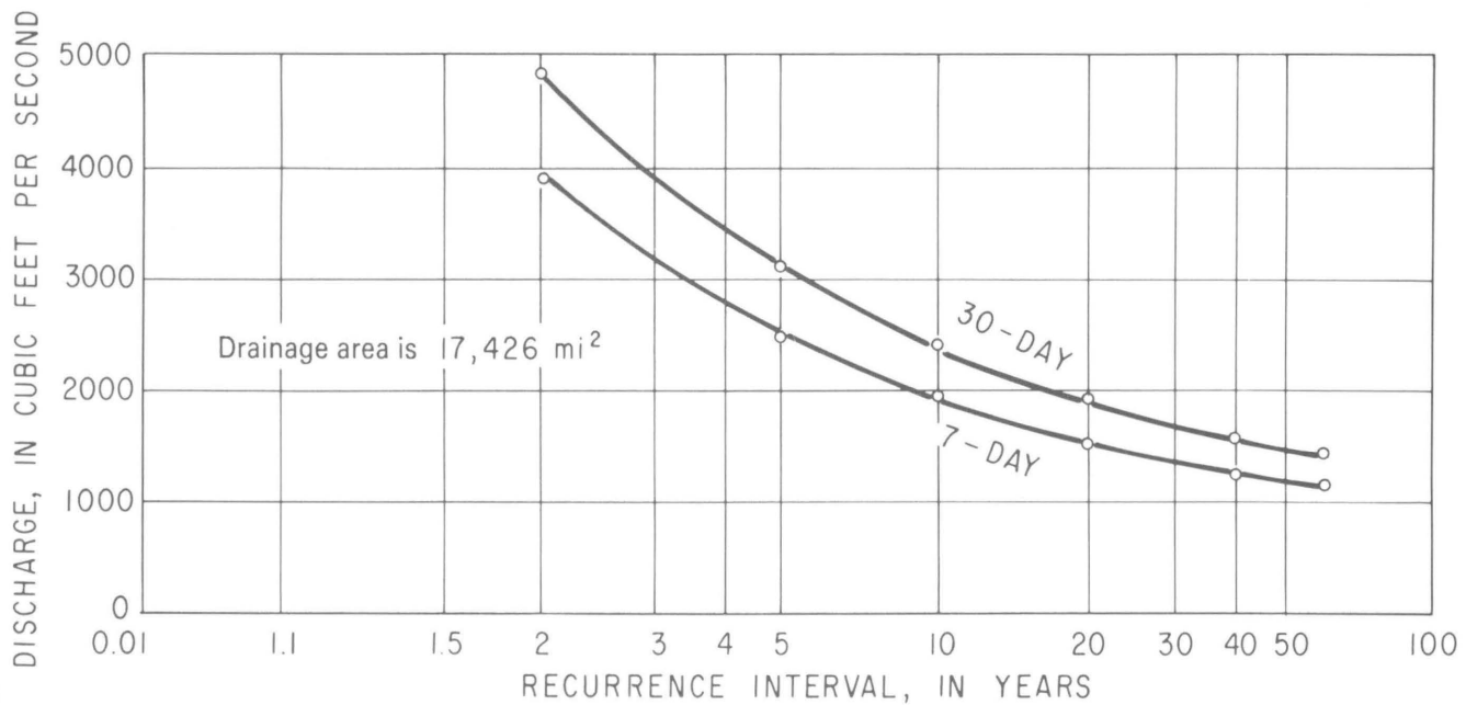
Figure 4.4. Minimum 7- and 30-consecutive-day average inflow to Albemarle Sound from land drainage (not adjusted for precipitation on and evaporation from open-water areas).
