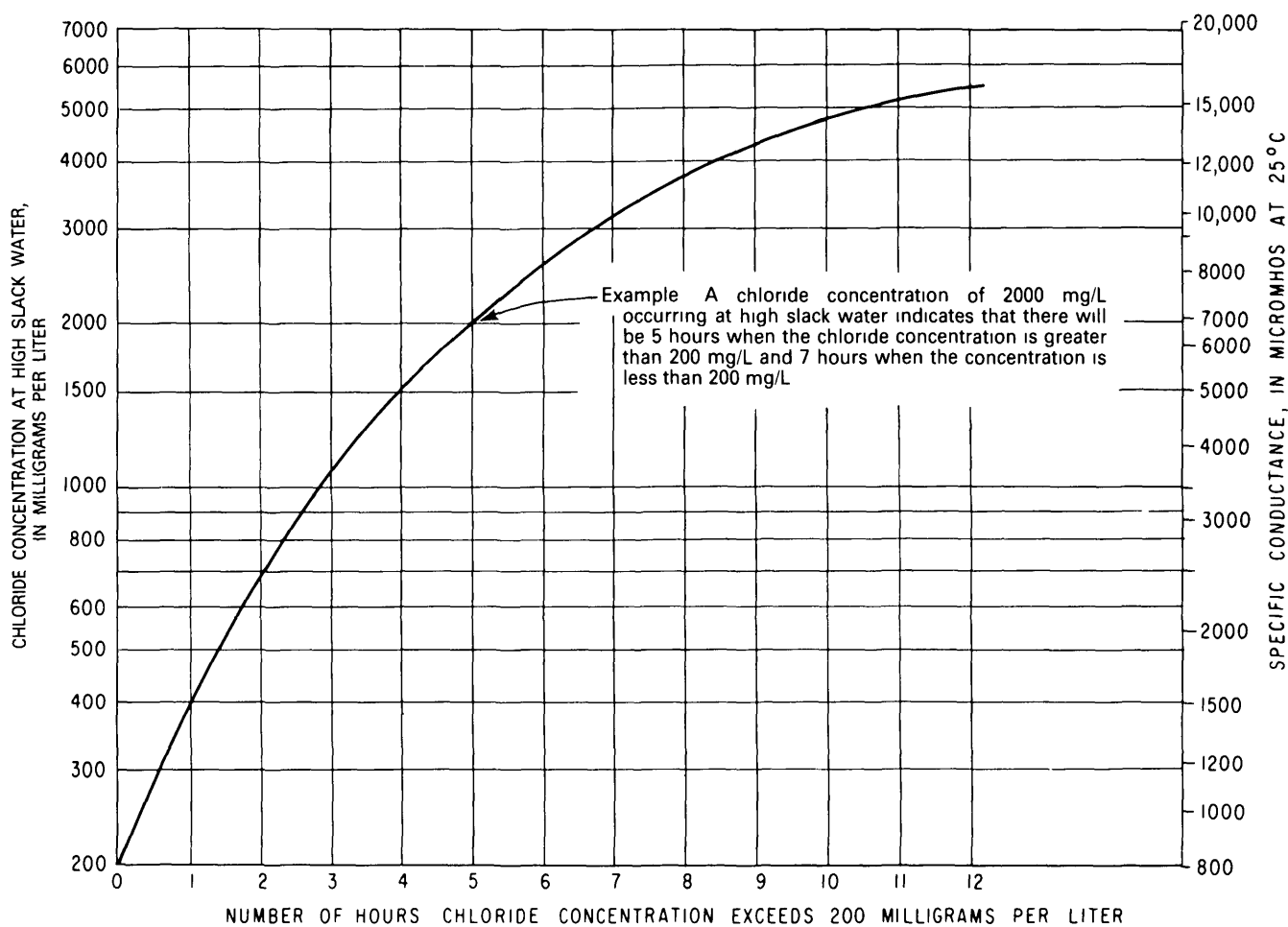
Figure 2.9. Relation between chloride concentration near the bottom of the Cape Fear River estuary upstream from Wilmington at high slack water and the number of hours the chloride concentration will exceed 200 mg/L near the channel bottom (From Wilder and Hubbard, 1968)
