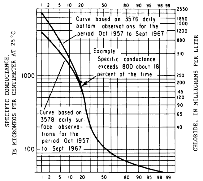
PERCENTAGE OF TIME SPECIFIC CONDUCTANCE OR CHLORIDE CONCENTRATION IS EQUAL TO OR GREATER THAN A GIVEN VALUE
