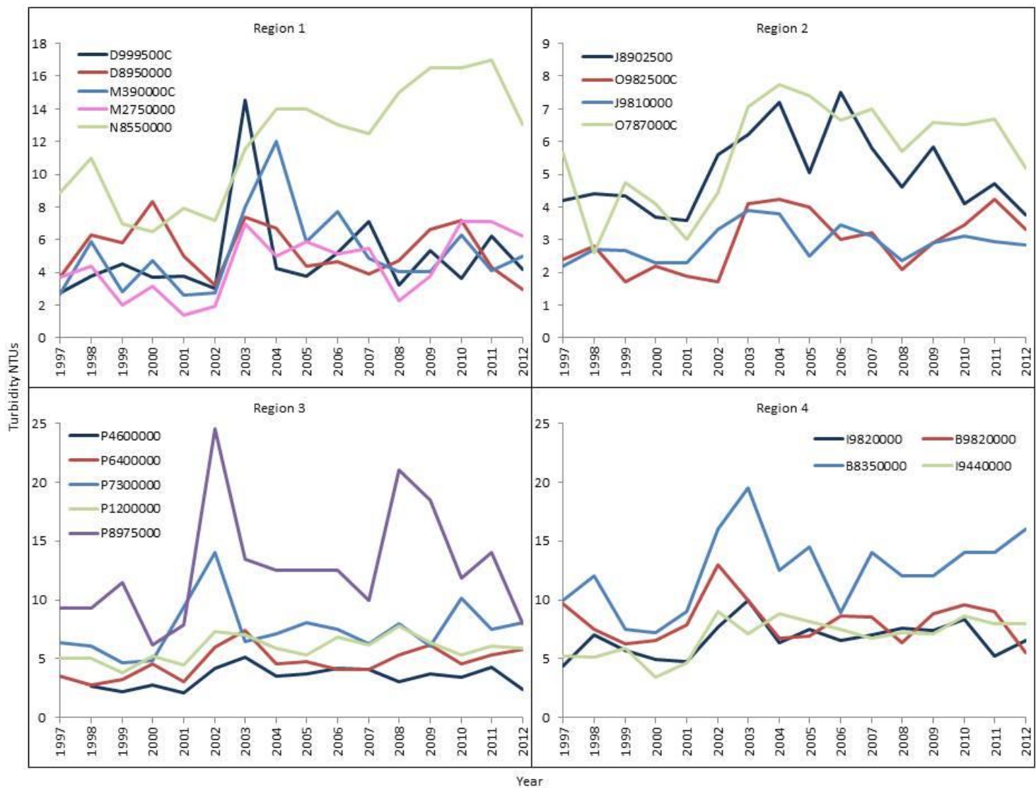
Figure 2.4f. Median values of Turbidity NTUs from 18 representative DWR ambient stations throughout the CHPP management area. See Map 2.3 for station location. These graphs are not statistical trends or meant to show standard exceedance, but are generated to show general trends over the last ~15 years.
