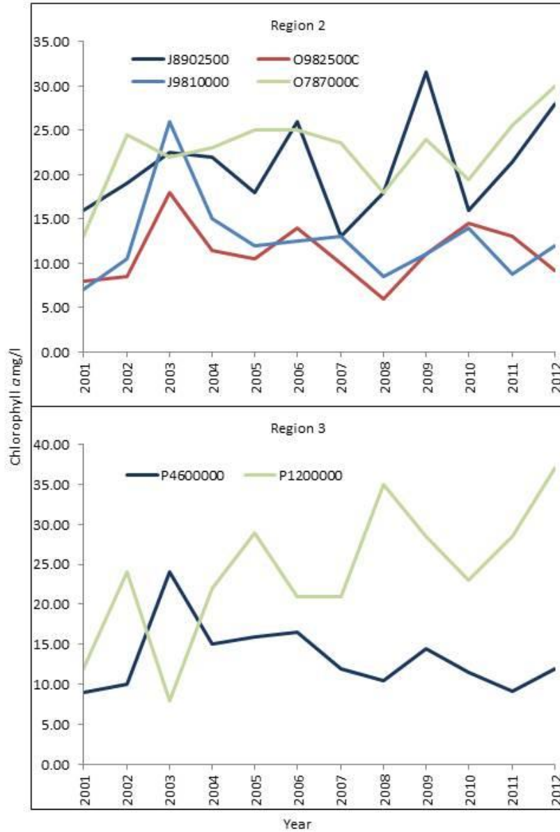
Figure 2.4a. Median values of Chlorophyll a mg/l from 18 representative DWR ambient stations throughout the CHPP management area. See Map 2.3 for station locations. These graphs are not statistical trends or meant to show standard exceedance, but are generated to show general trends over the last ~15 years.
