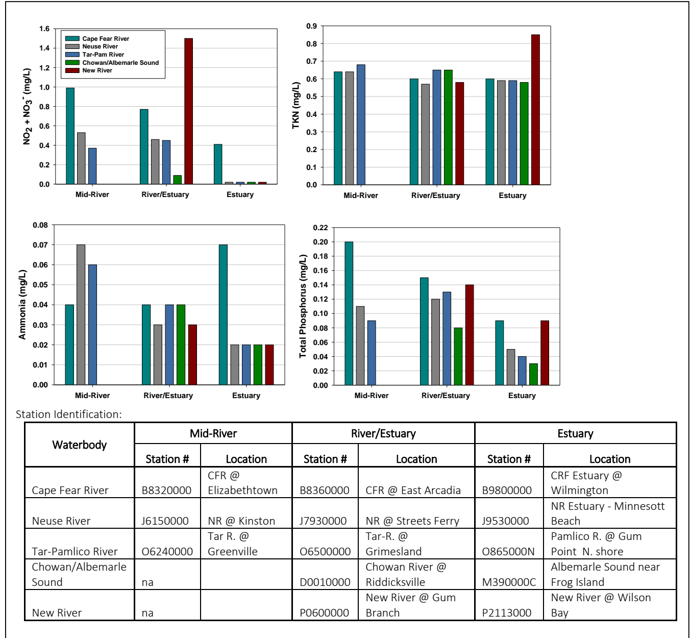
Figure 10.5. Median Nutrient Concentration Comparison within the Riverine, Estuarine Headwaters (River/Estuary) and Estuarine Systems in the Coastal Plain.
